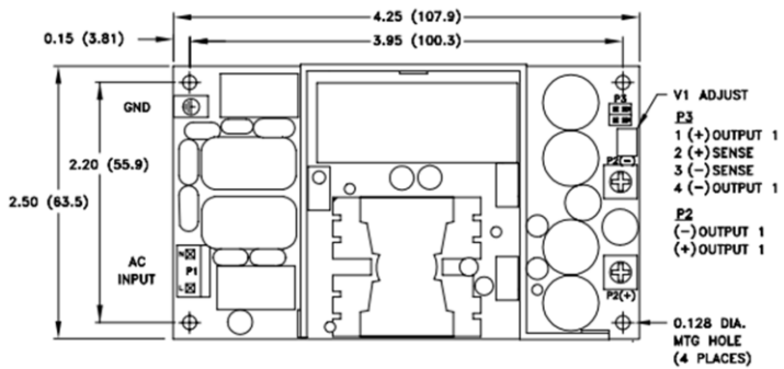
OPEN FRAME
