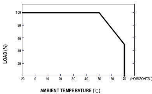
Derating Curve
