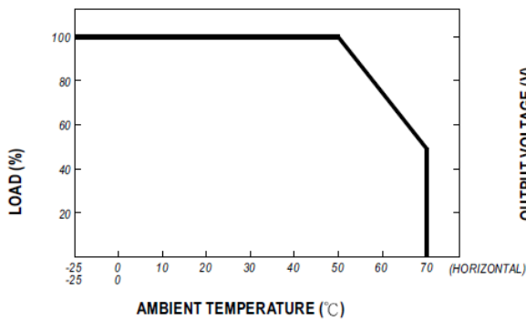
Load vs Ambient Temperature
