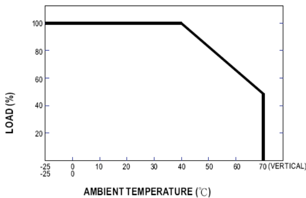
Derating Curve
