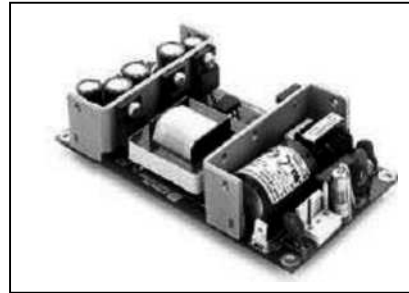
(size 101.6 x 57.2 x 23.6 mm including component lead throughs)
