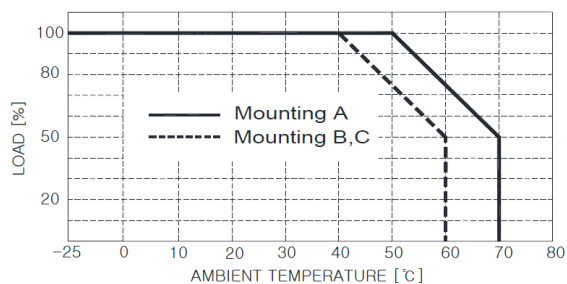
Load vs Ambient Temperature
