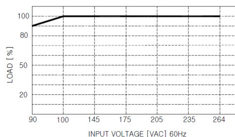
Load vs Input Voltage
