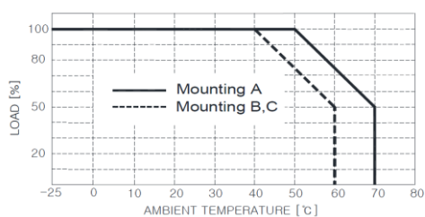
Load vs Ambient Temperature Load vs Input Voltage
