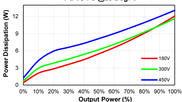
CQB75-300S3V3 Pd Vs Po @25 Deg. C
