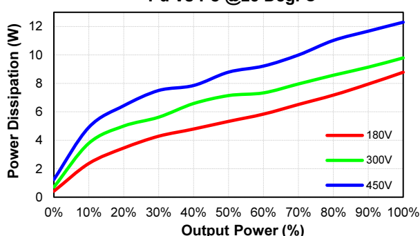
CQB75-300S12 Pd Vs Po @25 Deg. C
