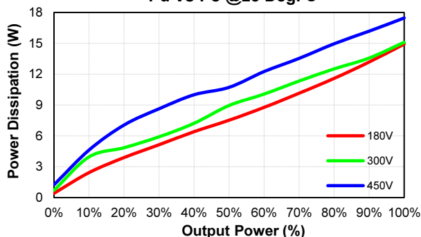
CQB75-300S05 Pd Vs Po @25 Deg. C
