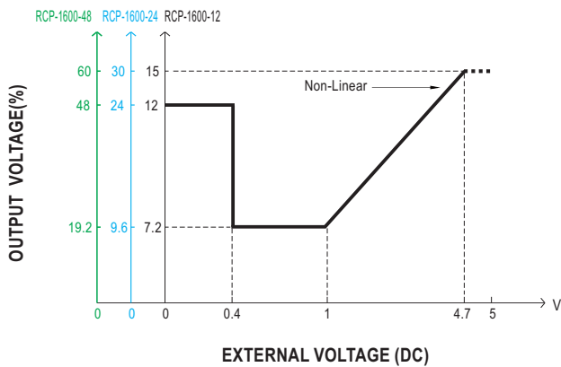
◎ For power supply system
