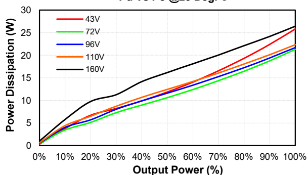
CHB200W-110S24-CMFC Pd Vs Po @25 Deg. C
