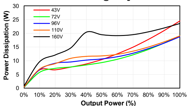
CHB200W-110S12-CMFC Pd Vs Po @25 Deg. C
