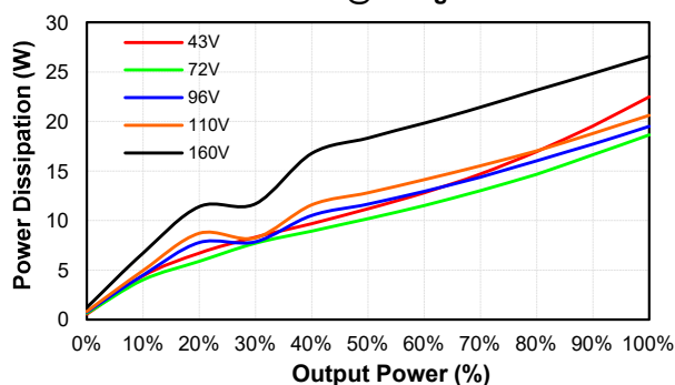
CHB200W-110S48-CMFC Pd Vs Po @25 Deg. C
