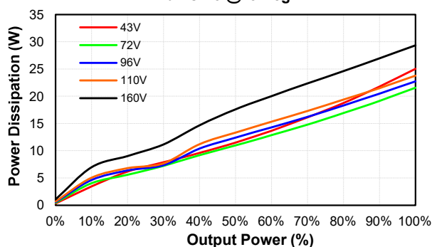
CHB200W-110S28-CMFC Pd Vs Po @25 Deg. C
