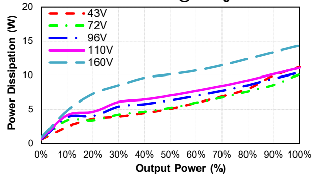
CQB100W-110S48-CMFC Pd Vs Po @25 Deg. C
