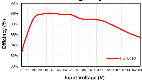
EC7BW18-72D24 Eff Vs Io @25 Deg. C
