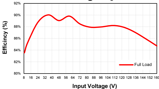
EC7BW18-72S12 Eff Vs Io @25 Deg. C
