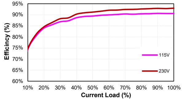
CBM150S360 (Eff Vs Io)
