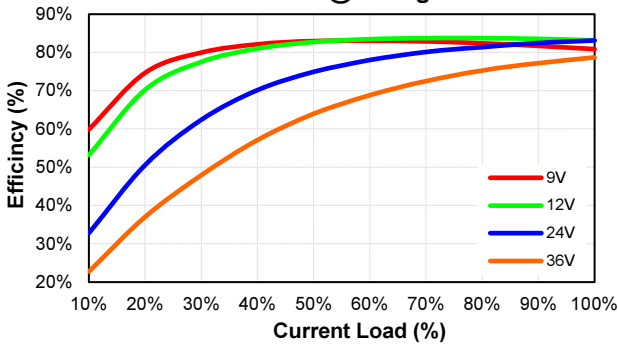
EC3SAW-24S12HP Eff Vs Io @25 Deg. C
