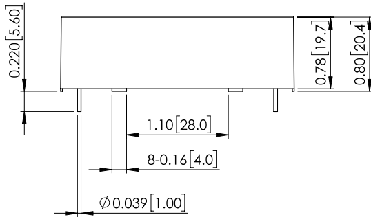
CFM21SXXX-S
