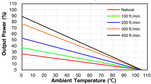
CHB500W-24SXX Derating Curve without Heatsink (Vin=24V)
