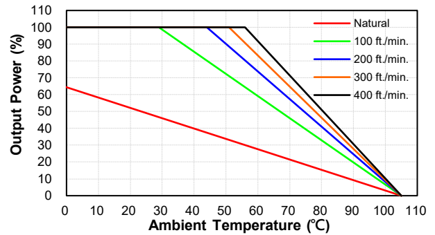
CHB500W-24SXX Derating Curve with Heatsink HBT254 (Vin=24V)
