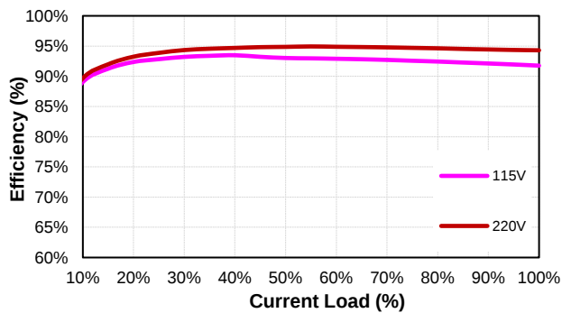
LFM550S240 (Eff Vs Io)
