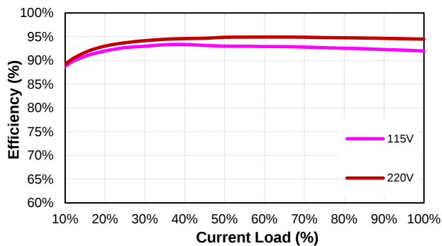
LFM550S300 (Eff Vs Io)
