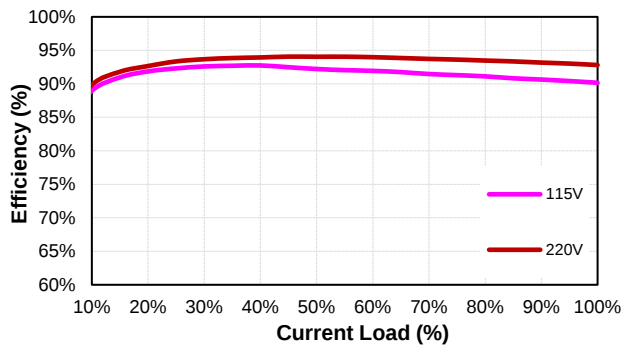
LFM550S120 (Eff Vs Io)
