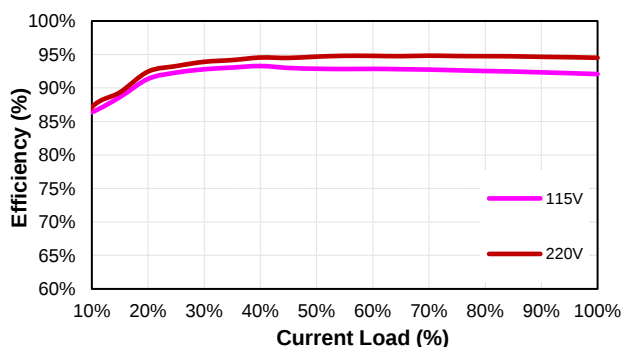
LFM550S480 (Eff Vs Io)
