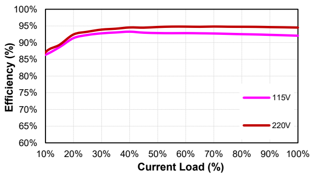
LFM550M480 (Eff Vs Io)
