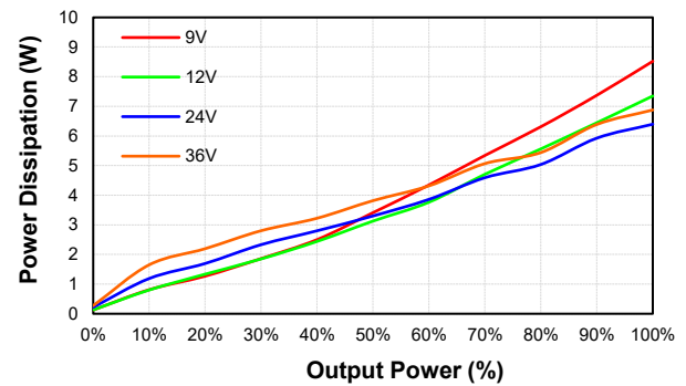
CQM60W-24S24 Pd Vs Po @25 Deg. C
